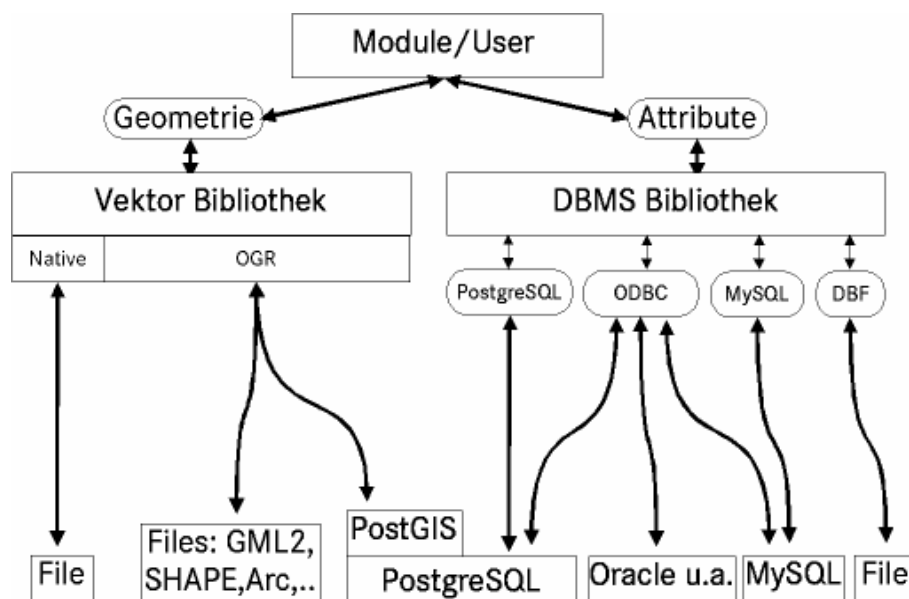
Abb. 3: Vektordatenmanagement in GRASS GIS
